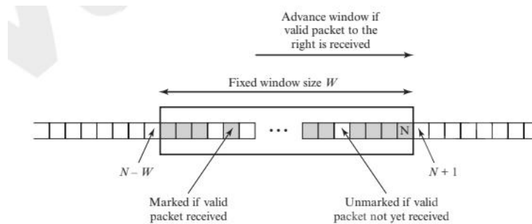
Figure 20.6 Anti-replay Mechanism
