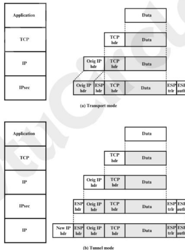
Figure 20.9 Protocol Operation for ESP
