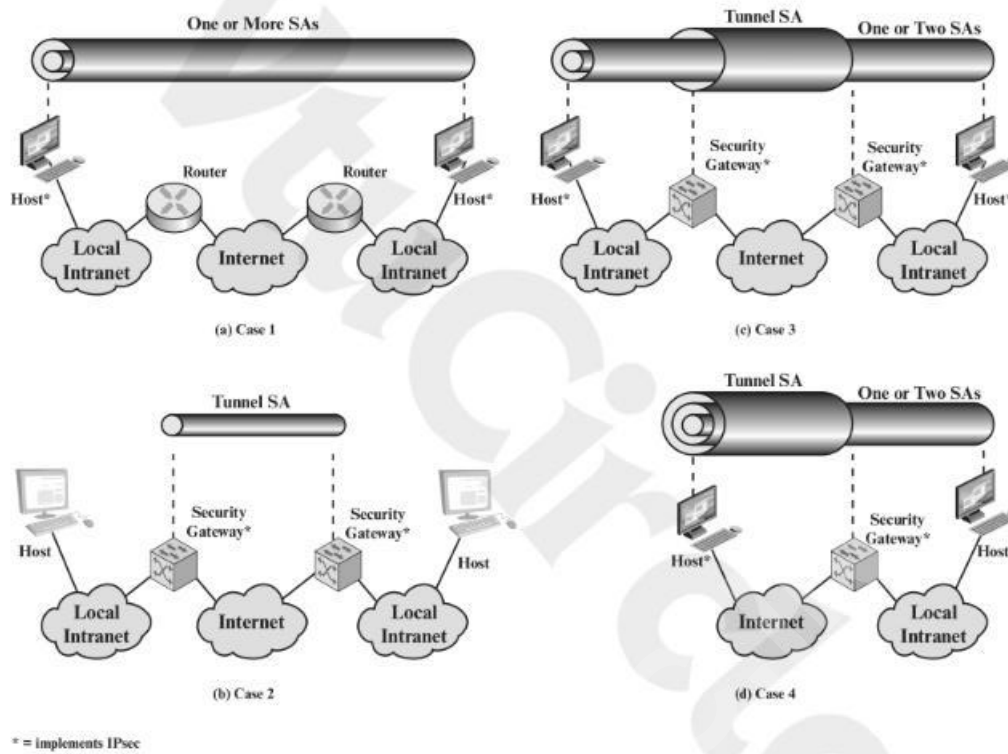
Figure 20.10 Basic Combinations of Security Associations
