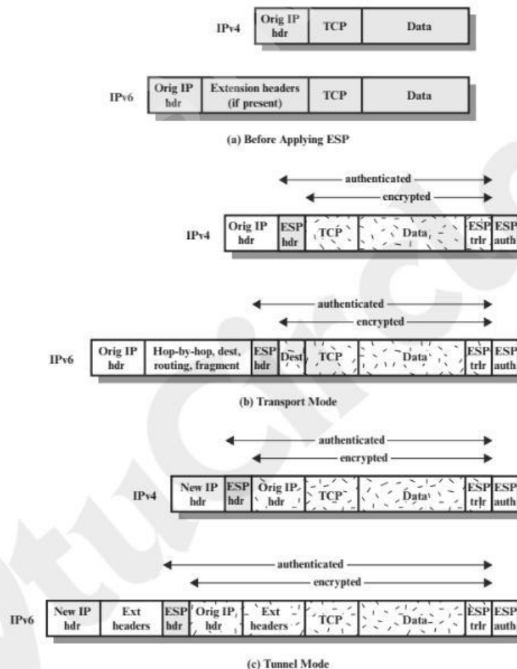
Figure 20.8 Scope of ESP Encryption and Authentication
