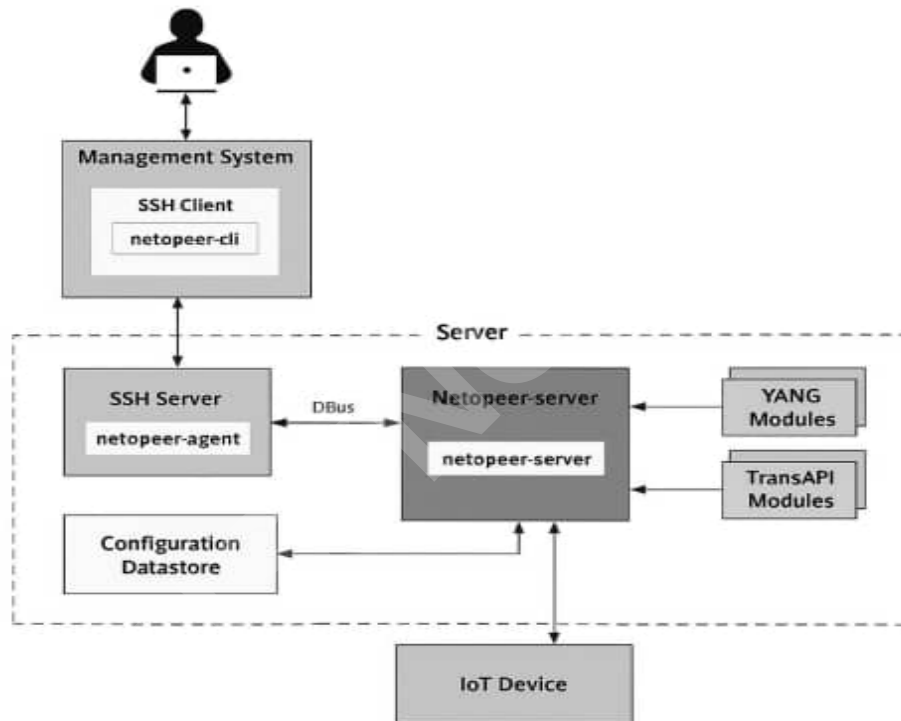
Figure 4.6: IoT device management with NETCONF - a specific approach based on Netopeer tools
