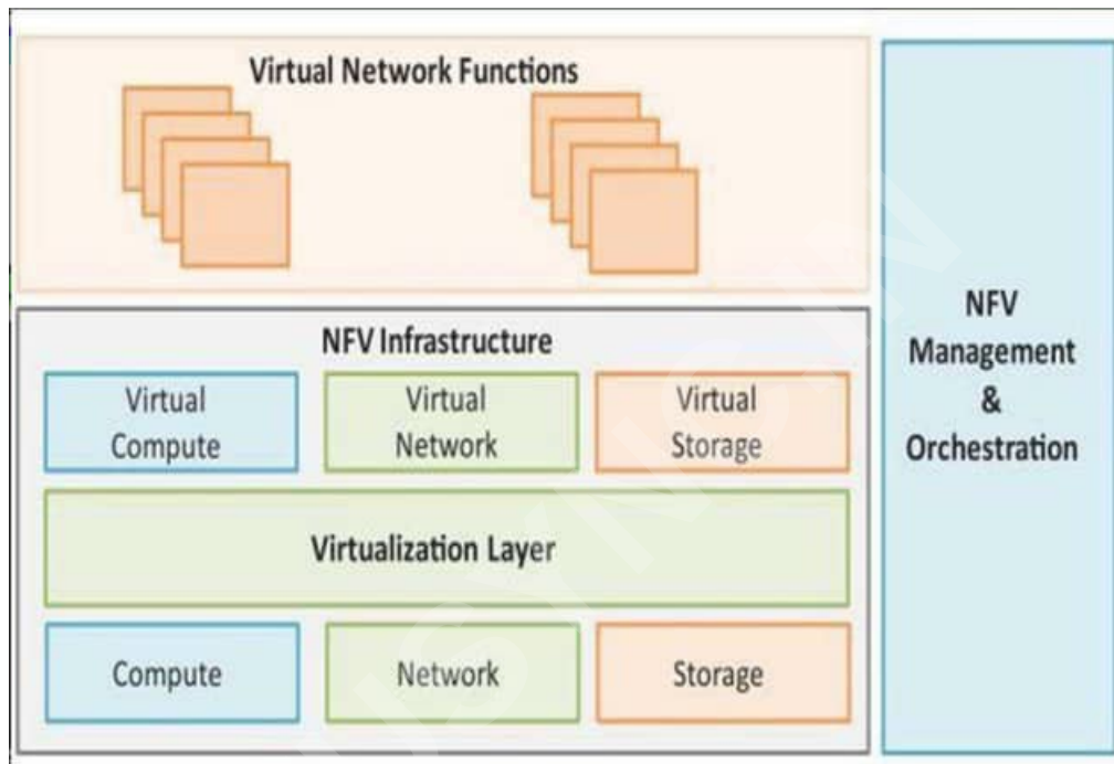
Figure 3.11: NFV architecture
