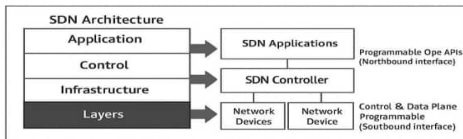
Figure 3.8: SDN layers
