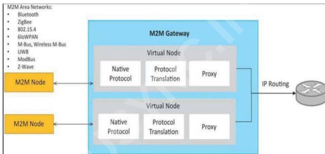
Figure 2.2: block diagram of an M2M gateway.
