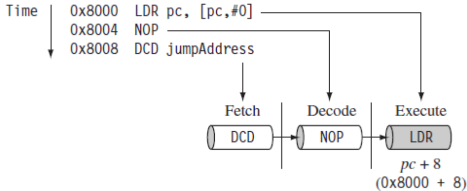
Figure: Example: pc = address + 8
