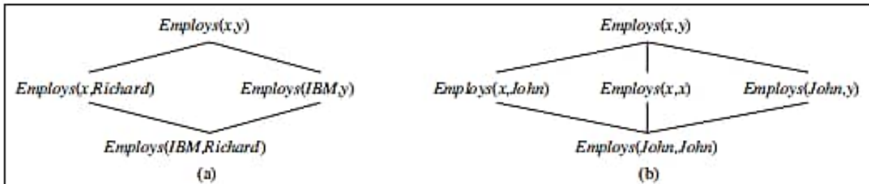
Figure 9.2 (a) The subsumption lattice whose lowest node is Employs(IBM, Richard) . (b) The subsumption lattice for the sentence Employs(John, John) .
