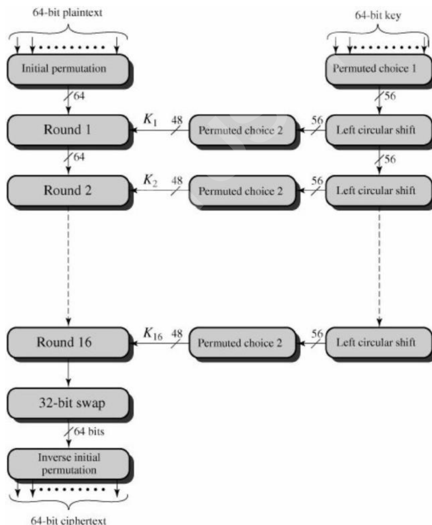
Figure 3.4. General Depiction of DES Encryption Algorithm
