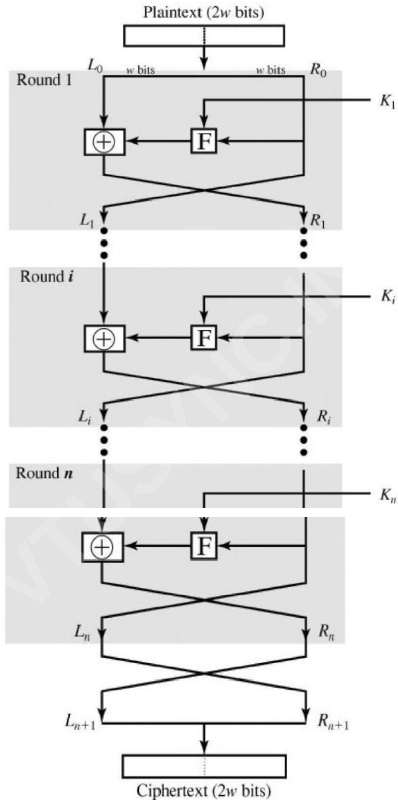
Figure 3.2. Classical Feistel Network
