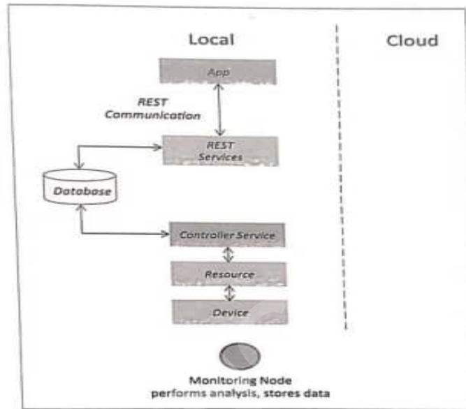
Figure 5.9: Deployment design of the home automation IoT system
