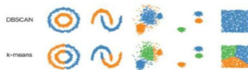
FIGURE 2.25 DBSCAN and k-means Clustering Algorithms
