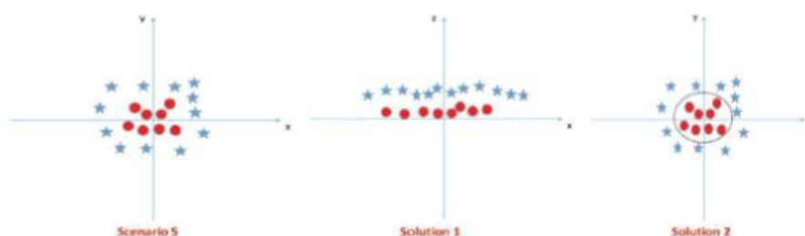
FIGURE 2.39 Evaluating Hyperplanes
