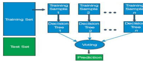
FIGURE 2.19 Random Forest
