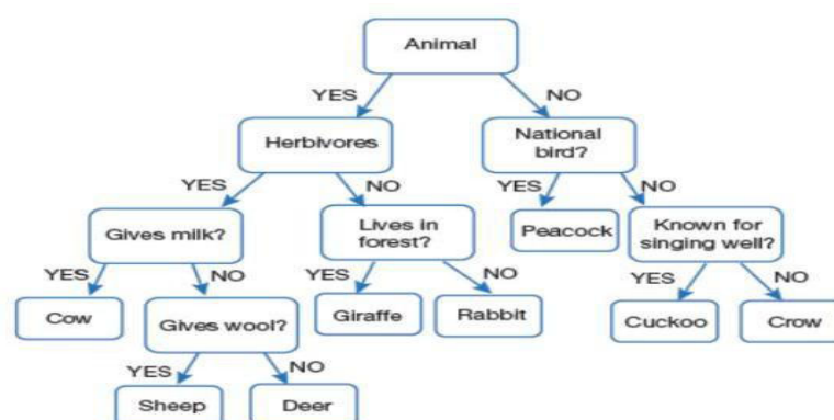
FIGURE 2.17 Decision Tree
