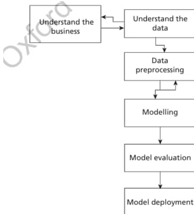
Figure 1.11: A Machine Learning/Data Mining Process
