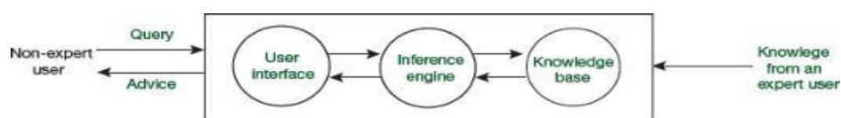
FIGURE 9.7 Participants in an expert system
