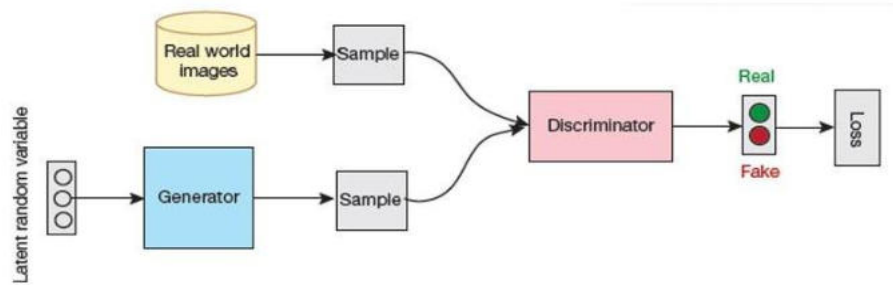
FIGURE 8.22 GAN Architecture [3]
