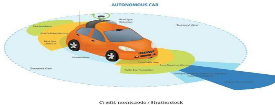
FIGURE 9.12 Autonomous Vehicle
