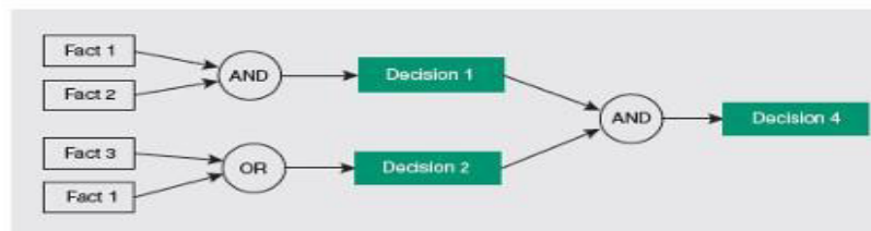
FIGURE 9.4 Forward Chaining
