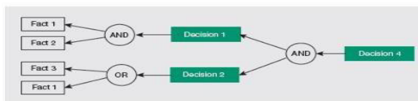
FIGURE 9.5 Backward Chaining
