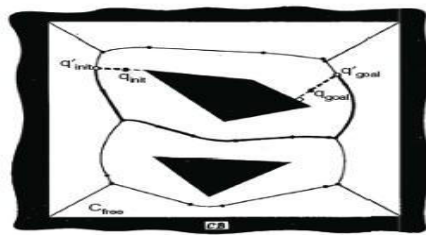
FIGURE 8.17 Voronoi Diagram
