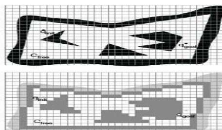
FIGURE 8.19 Exact Cell Decomposition
