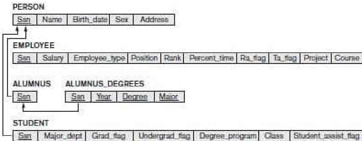
Figure 9.6 Mapping the EER specialization lattice in Figure 8.8 using multiple options.
