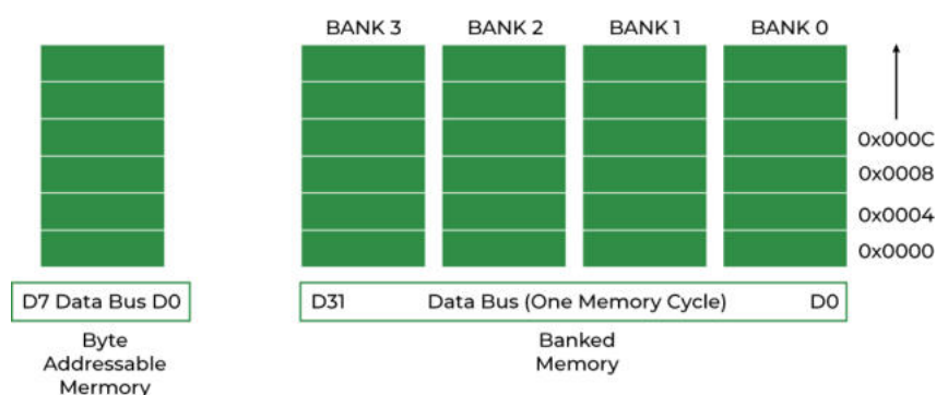
Fig 3.2 Data Alignment in Memory
