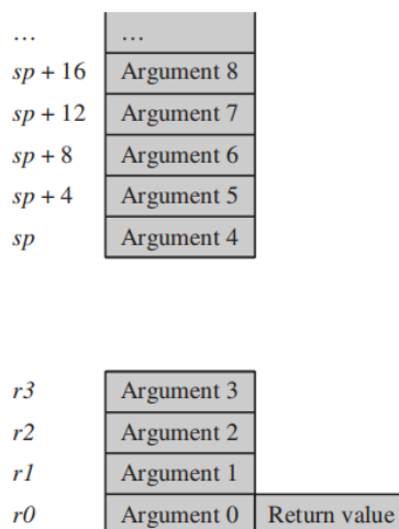
Fig 3.1 ATPCS argument passing.
