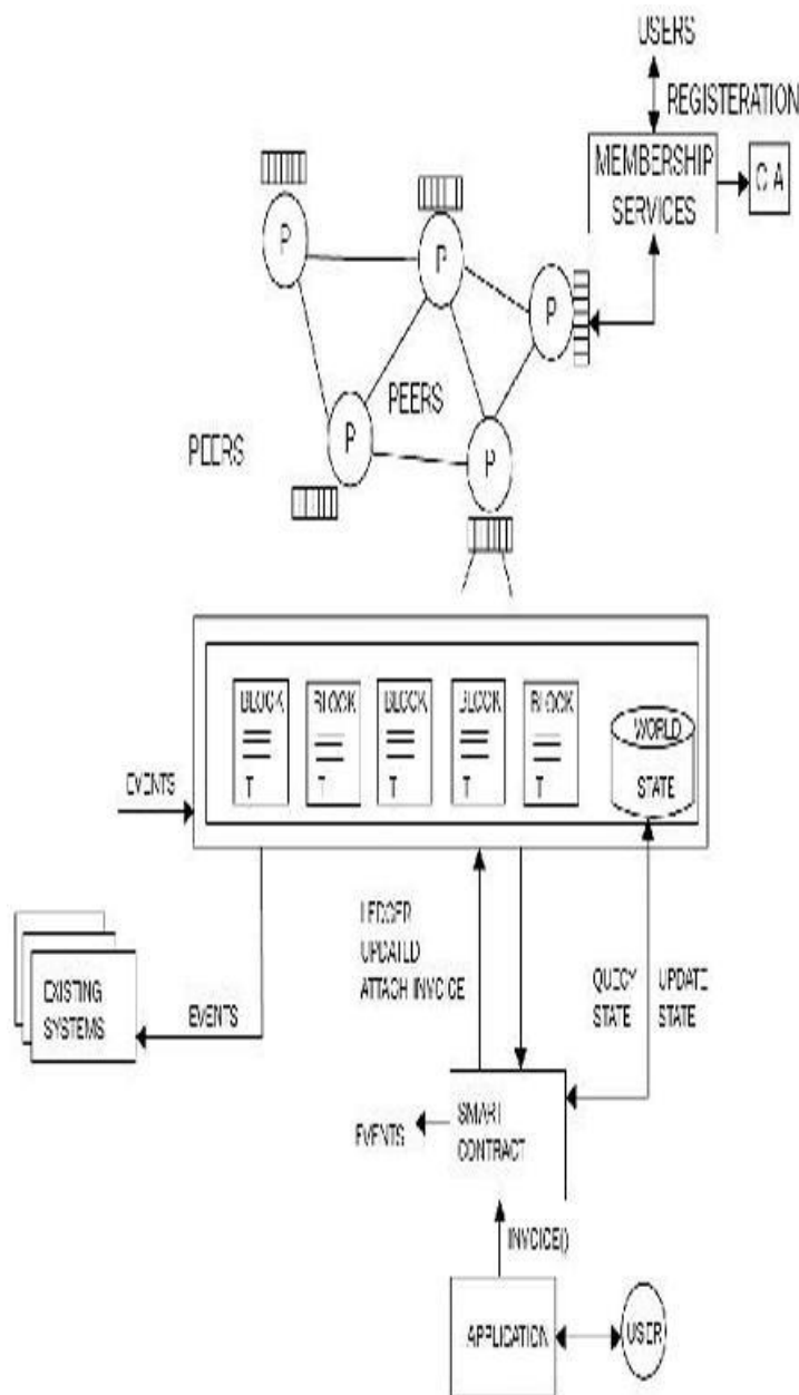
HIGH LEVEL OVERVIEW OF HYPERLEDGER FABRIC
