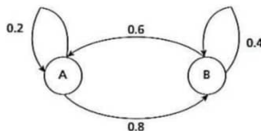
Figure 14.6: Markov Chain
