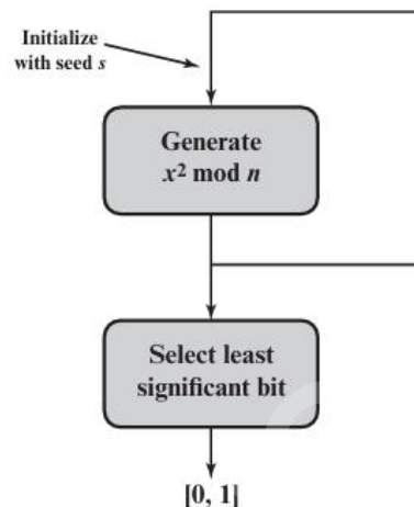
Figure 8.3 Blum Blum Shub Block Diagram
