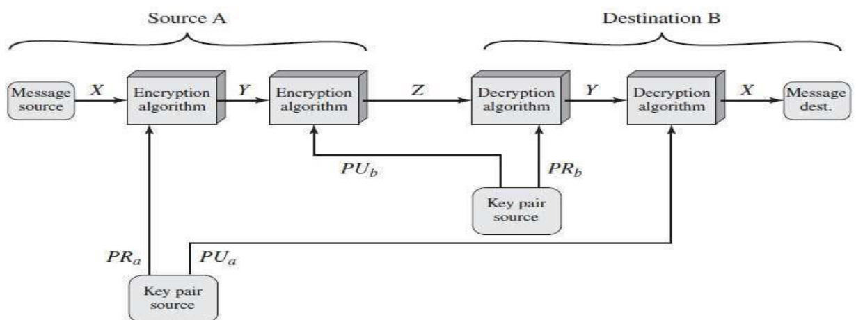
Figure 9.4 Public-Key Cryptosystem: Authentication and Secrecy
