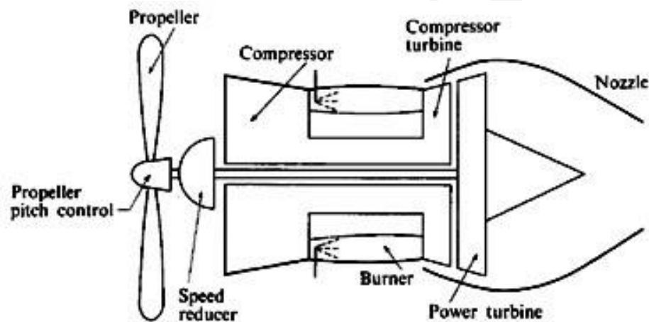
Fig: Turboprop engine
