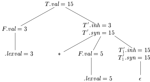
Figure 5.5: Annotated parse tree for 3 * 5
