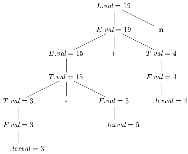
Figure 5.3: Annotated parse tree for 3 * 5 + 4 \mathbf{n}
