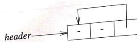
(a) Zero polynomial
