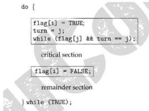
Figure: The structure of process P_i in Peterson's solution.
