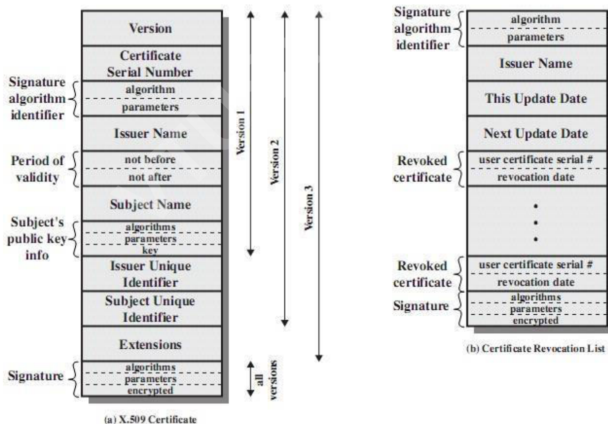
Figure 14.4 X.509 Formats
