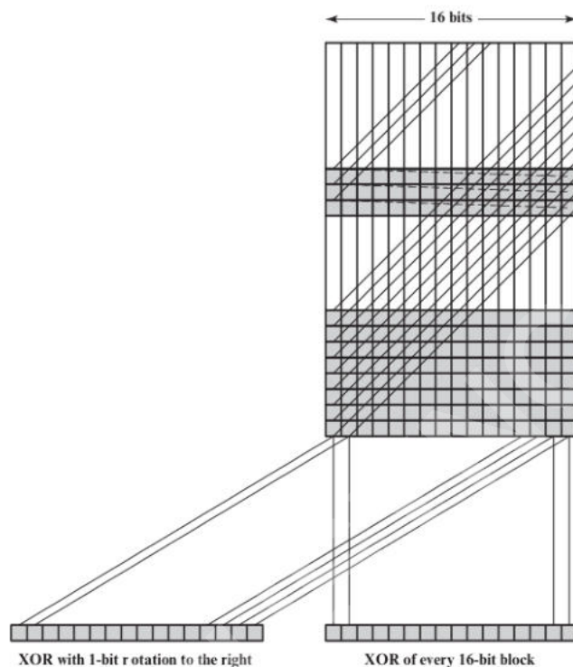
Figure 11.5 Two Simple Hash Functions
