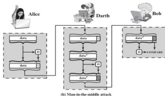
Figure 11.2 Attack Against Hash Function
