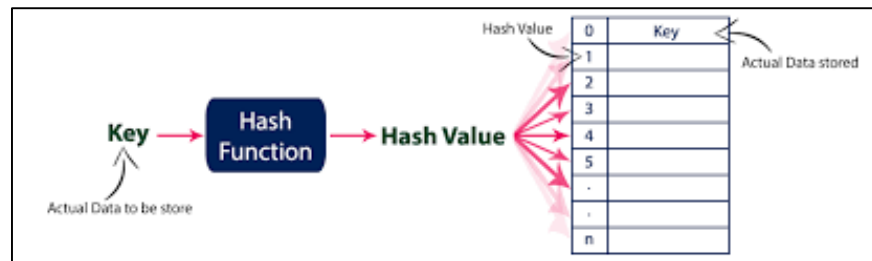
Figure 5.17 Hashing.
