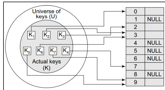
Figure 5.18 Collision Example
