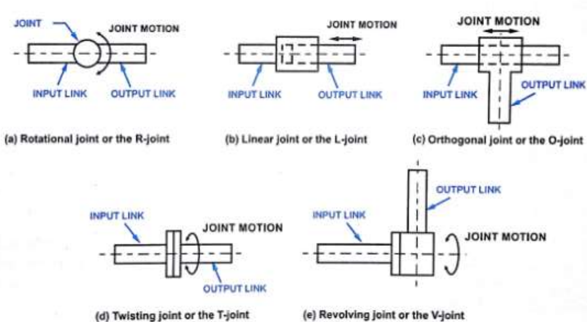
Types of Robot joints
