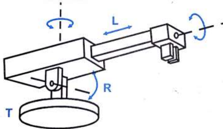
Polar Configuration Robot
